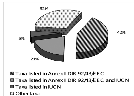
Fig. 2 - Percentages of papers related to the taxa listed in Annex II Directive 92/43/EEC and in the IUCN Red List 2009 under CR category.
